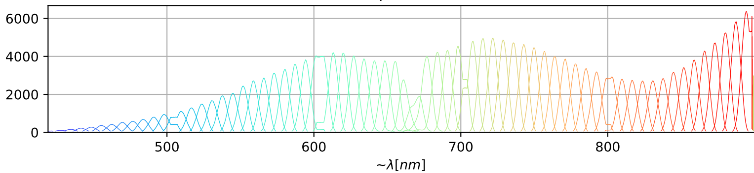
VNIR SRF - spatial column 961
