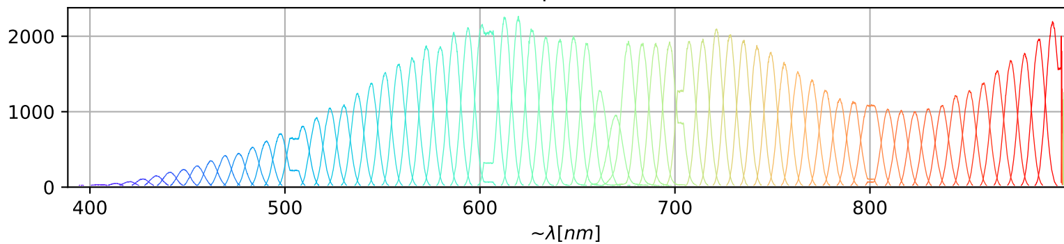
VNIR SRF - spatial column 360
