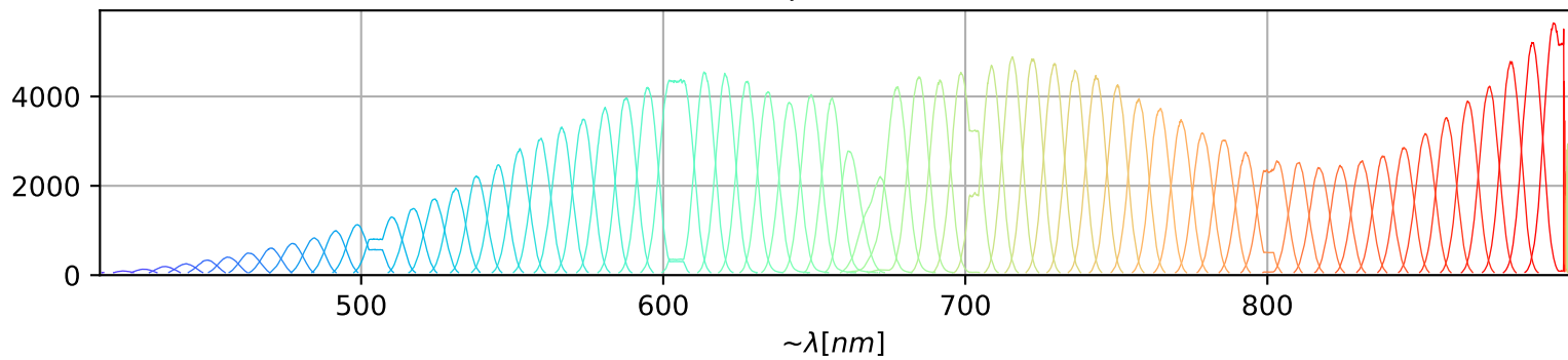
VNIR SRF - spatial column 637
