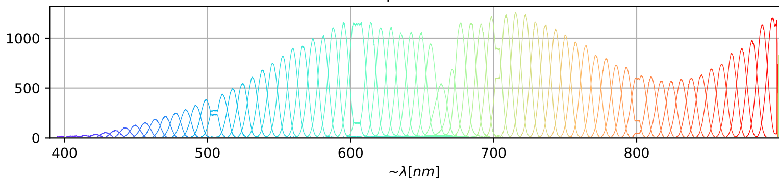
VNIR SRF - spatial column 1214
